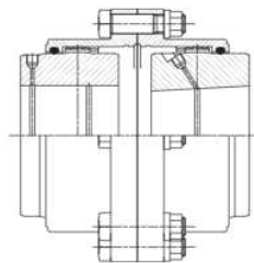
INTERFERENCE FIT
